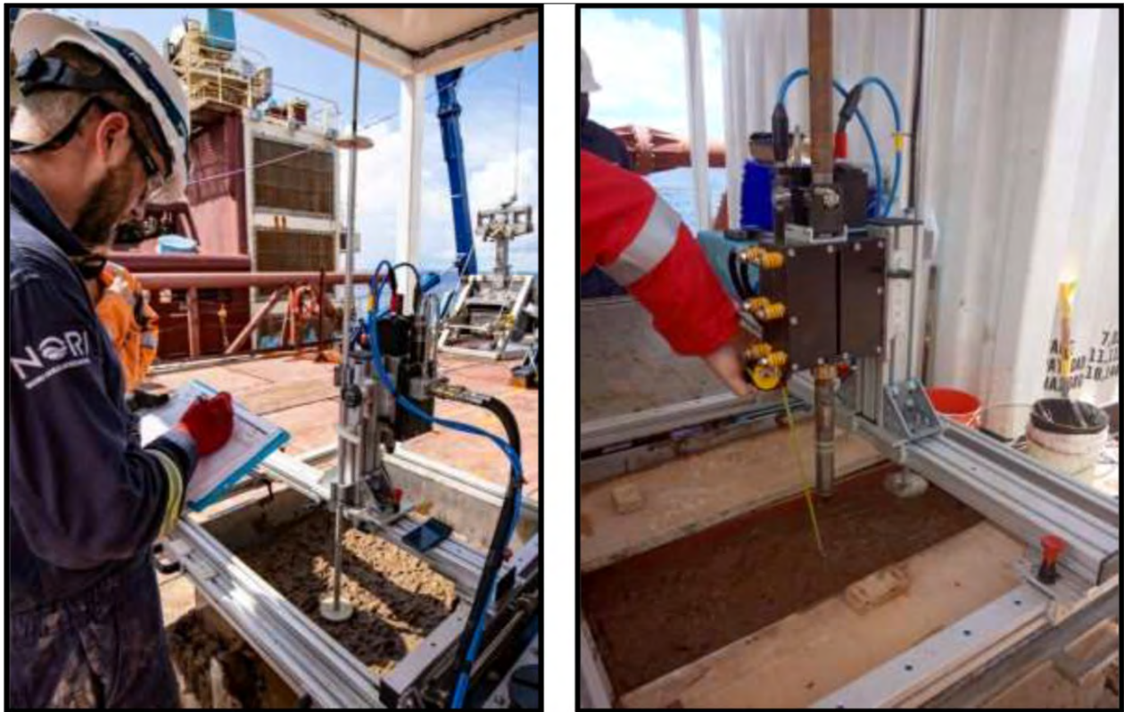
Figure 7.30 Photographs of geotechnical plate load test (left) and CPT (Right)
