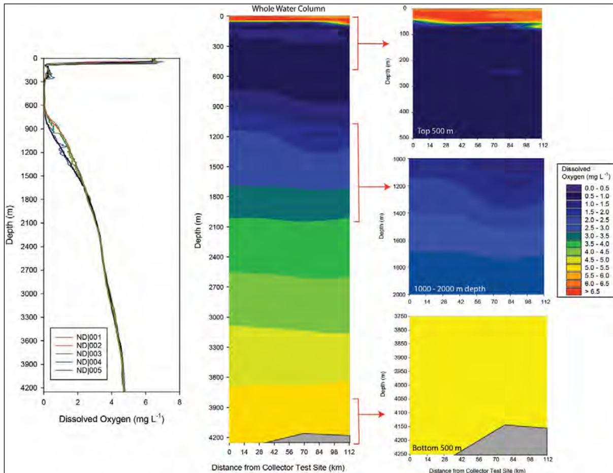
Figure 17.7 Dissolved oxygen ( \text{mg L}^{-1} ) profile of NORI Area D during Campaign 4A
