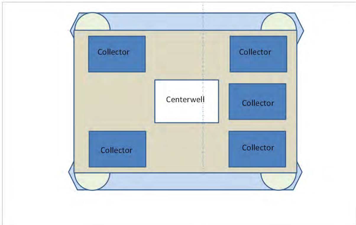
Figure 13.20 Deck plan for collector support vessel
