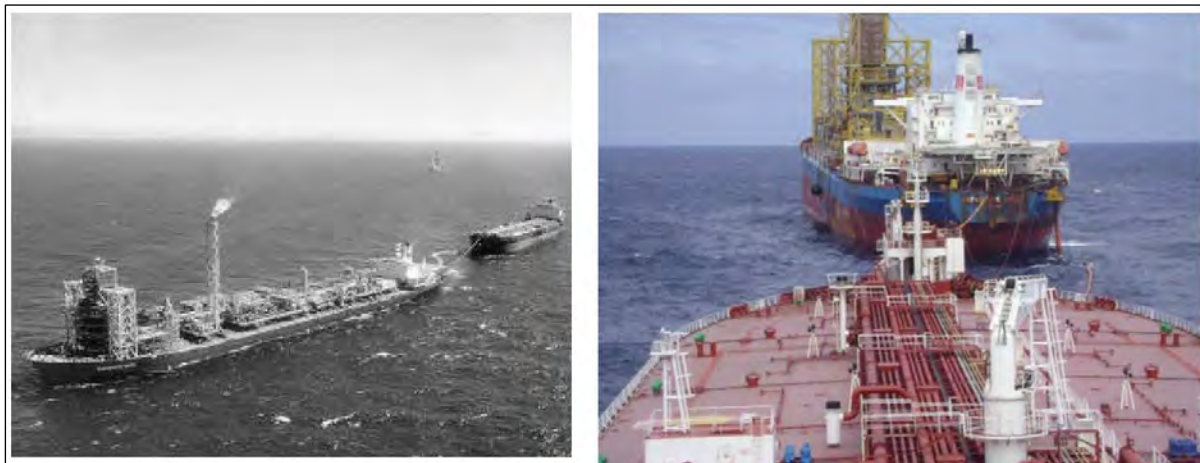
Figure 15.2 Offloading Operation: (left) with a conventional tanker; (right) with a DP tanker
